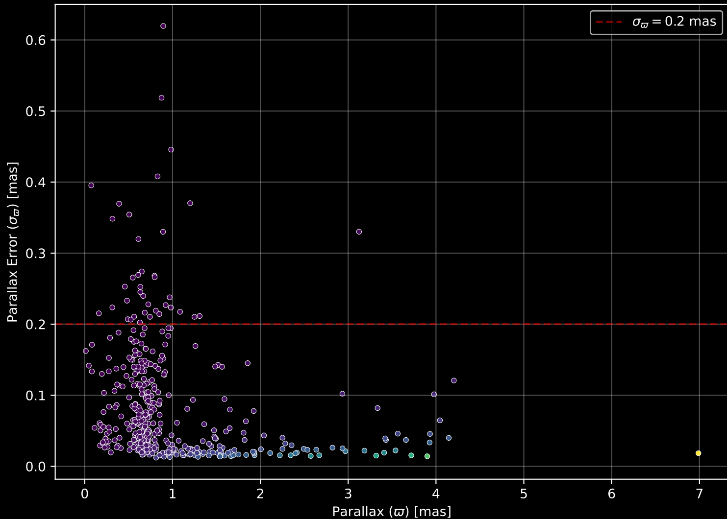
APOGEE DR17 Field: [Rosette_btx] Parallax Quality (n= 415)
